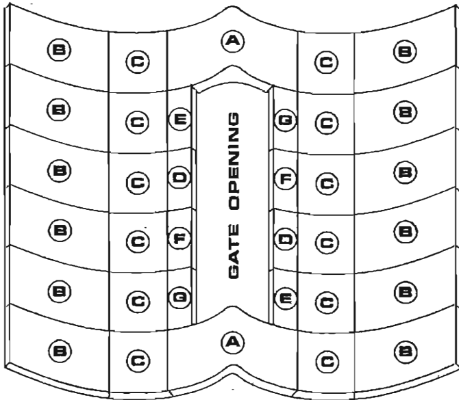
SHELL LINERS
