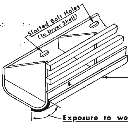
"EXTRA WEAR" Flights
