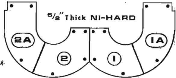
SPLIT END LINERS
