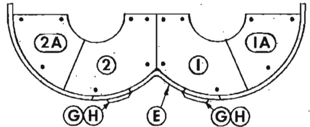
SPLIT END LINERS (5/8" Thick NI-HARD)
