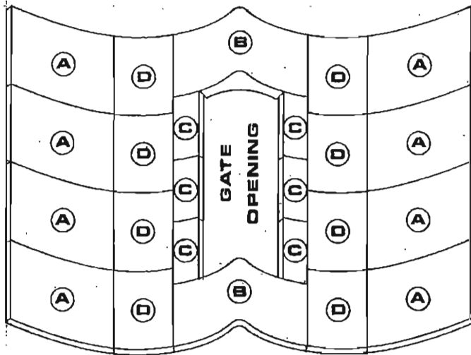
SHELL LINERS (3/4" Thick NI-HARD)
