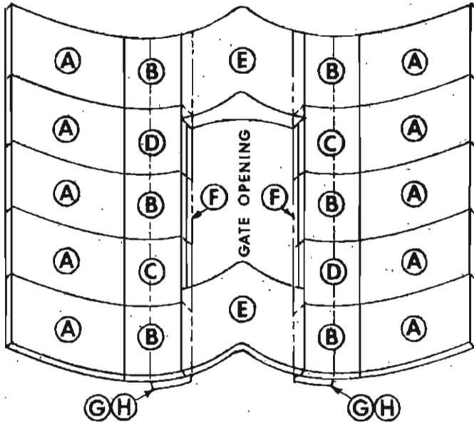
SHELL LINERS (3/4" Thick NI-HARD)
