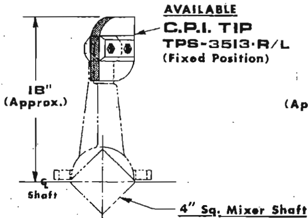
CEDARAPIDS MIXER ARM
