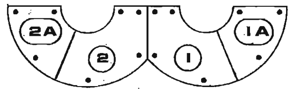
SPLIT END LINERS (5/8" Thick NI-HARD)
