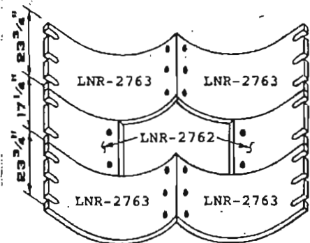
SHELL LINERS
