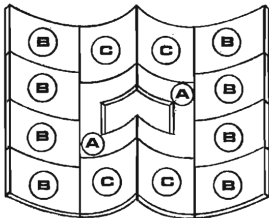
SHELL LINERS (3/4" Thick NI-HARD)
