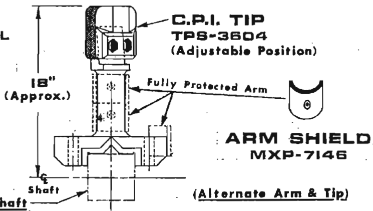
C.P.I. MIXER ARM SHK-3803-R/L
