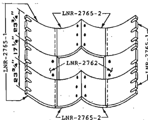
SPLIT SHELL LINERS (Alternate)
