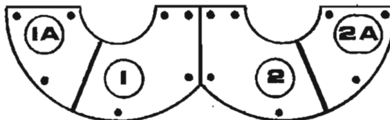
SPLIT END LINERS (3/4" Thick NI-HARD)
