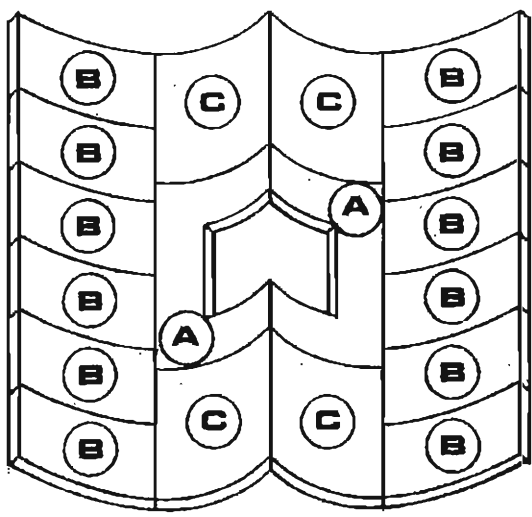
SHELL LINERS (3/4" Thick NI-HARD)
