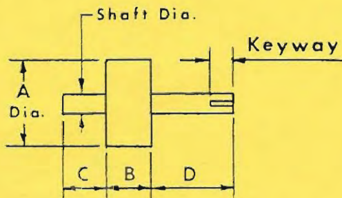
PLAIN TRUNNION (For Trunnion Drive)
