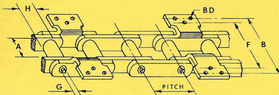
Chains with K-3 or K-35 Attachments
