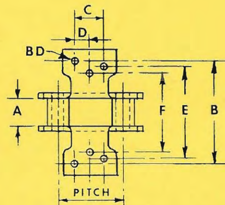
Chains with K-3 or K-35 Attachments
