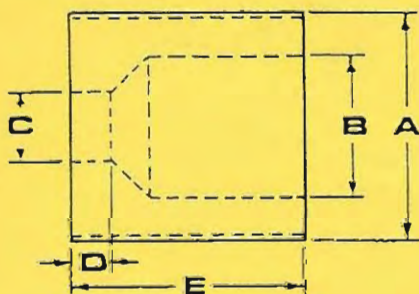
STRAIGHT CONE
