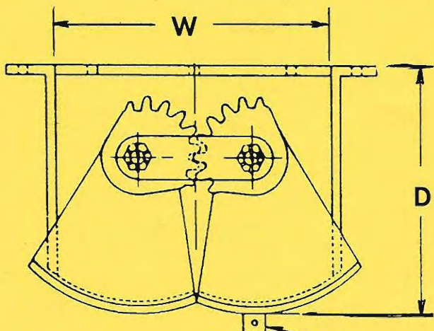
STYLE "DG"
