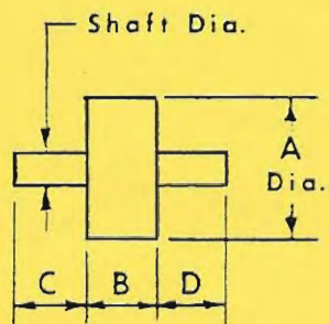
PLAIN TRUNNION (For Gear Drive)
