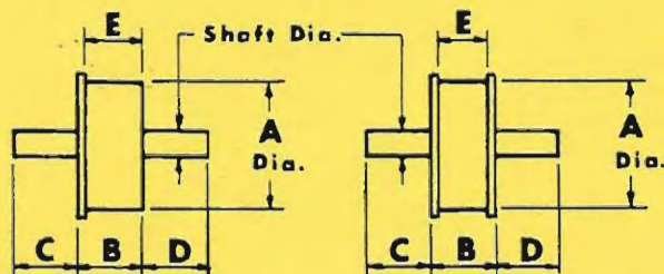
SINGLE FLANGE TRUNNION DOUBLE FLANGE TRUNNION
