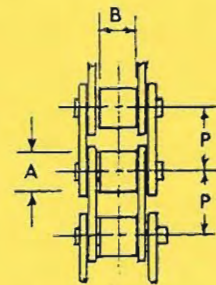
Single Strand
