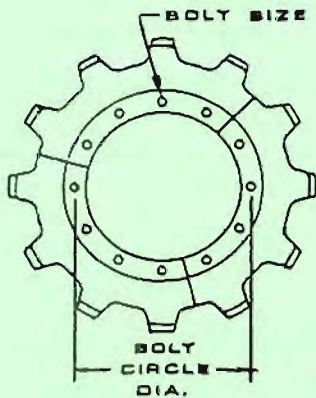
(3) SEGMENTS
