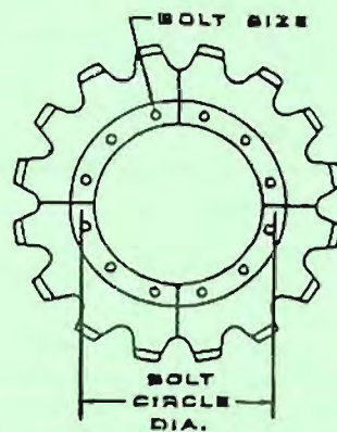
(4) SEGMENTS
