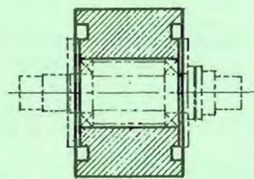
TRUNNION ROLLER
