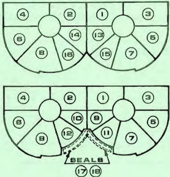
END LINERS
