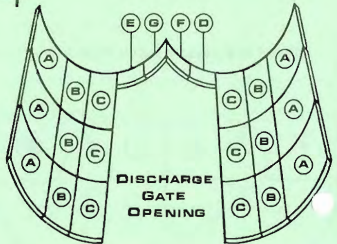
SHELL LINERS
